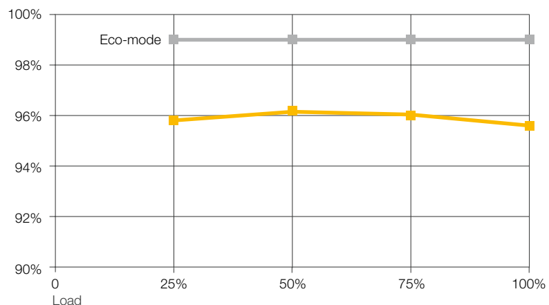
AC/AC Efficiency with linear, resistive load
